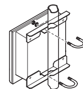
Pipe-mounting
