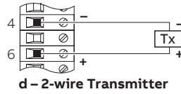
d – 2-wire Transmitter
